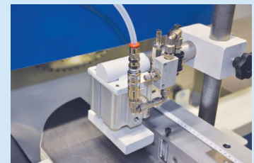
Vertical pneumatic clamp
