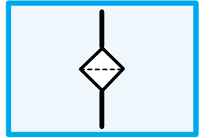
Filtro olio Oil filter Ölfiter
