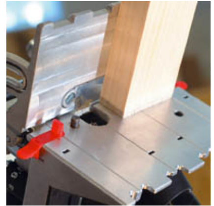
Thanks to the auxiliary stops, the edge spacing can be decreased or increased quickly and accurately.
