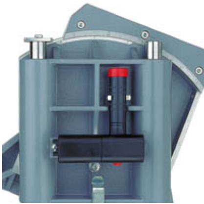
For cuts at an angle to the edge of the timber: tilt range up to 45° in both directions.
